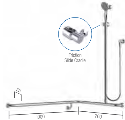
Drawn RH (Right Hand)
