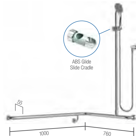
Drawn RH (Right Hand)
