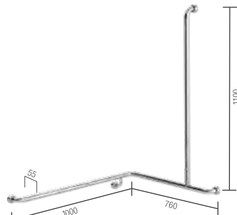
Drawn RH (Right Hand)
