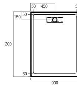
EL9012R 900x1200 Rear Outlet
