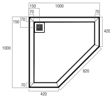
EC1000NR 1000x1000 Neo Corner Rear Outlet
