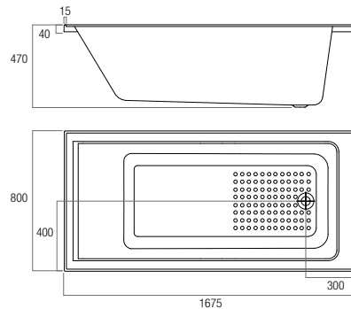
UB1675 1675x800x470
