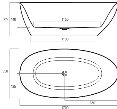
BOS1785 1700x850x585
