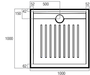
AS1000R 1000x1000 Rear Outlet
