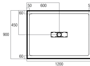
EL1290C 1200x900 Centre Outlet
