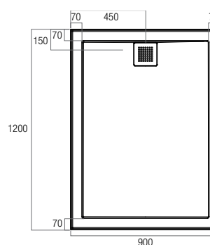
EC9012R 900x1200 Rear Outlet
