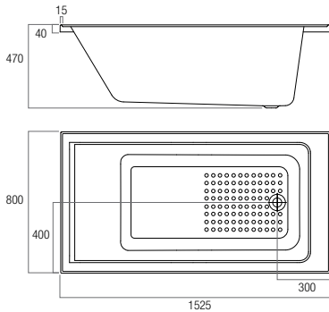
UB1500 1525x800x470
